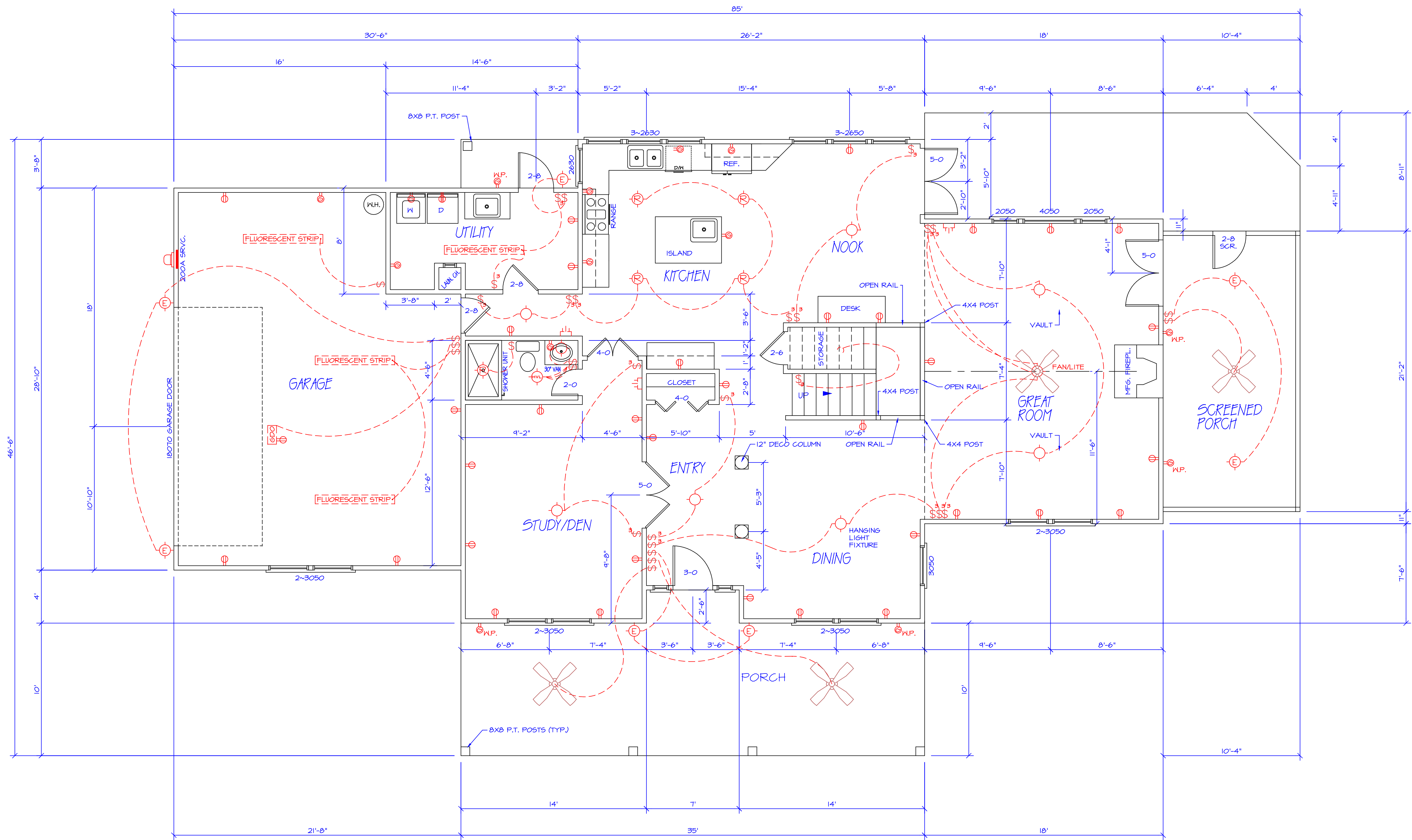
FIRST FLOOR PLAN SCALE: 1/4" = 1'-0" (1' CEILINGS)
